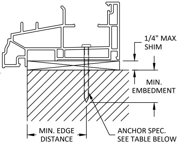
M 5 INSTALLATION DETAIL THROUGH FRAME SILL
