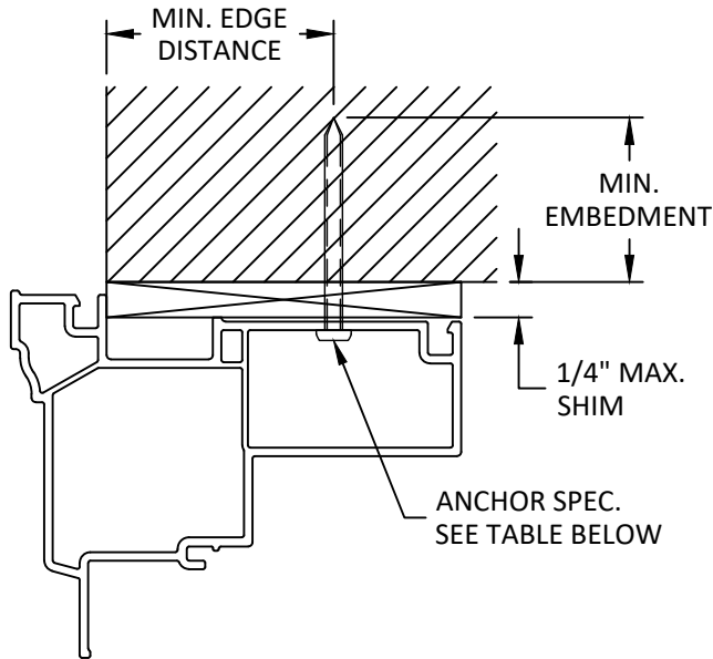
K 5 INSTALLATION DETAIL THROUGH FRAME HEAD
