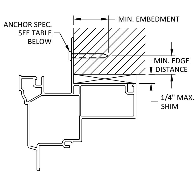
J 5 INSTALLATION DETAIL NAIL FIN HEAD
