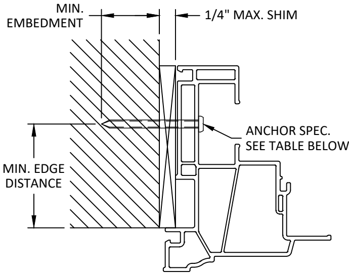
L 5 INSTALLATION DETAIL THROUGH FRAME JAMB
